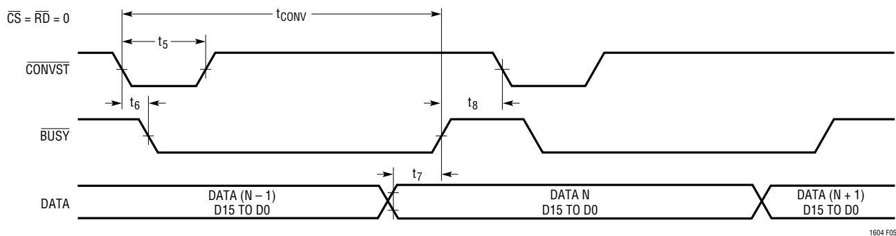
Figure 5. Mode 1a. \overline{CONVST} Starts a Conversion. Data Outputs Always Enabled ( \overline{CONVST} = \text{[Pulse]} \text{ )}
