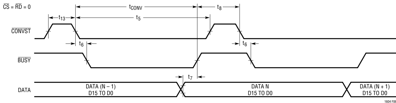
Figure 6. Mode 1b. \overline{CONVST} Starts a Conversion. Data Outputs Always Enabled ( \overline{CONVST} = \text{[Pulse]} \text{ )}
