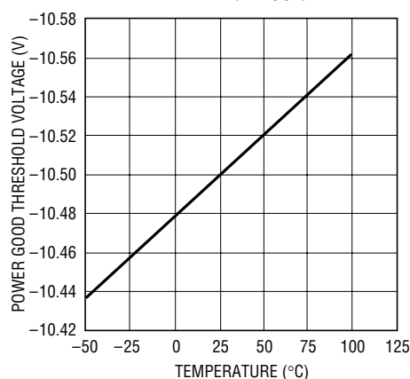
Power Good Threshold Voltage vs Temperature ( V_{\text{EEOUT}} )
