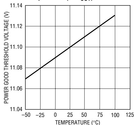
Power Good Threshold Voltage vs Temperature ( 12V_{\text{OUT}} )
