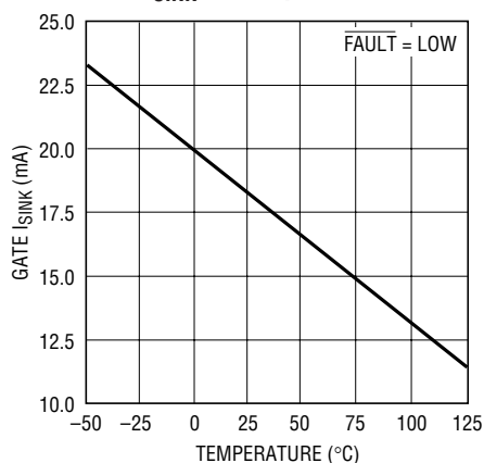
Gate I_{\text{SINK}} vs Temperature
