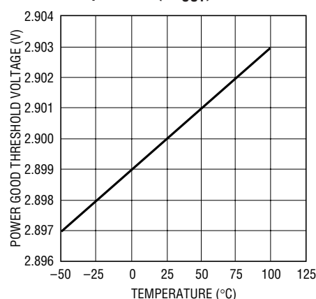
Power Good Threshold Voltage vs Temperature ( 3V_{\text{OUT}} )
