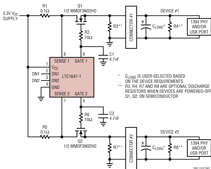
V IN Controller for Two Device Bays
