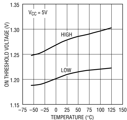
ON Threshold Voltage vs Temperature
