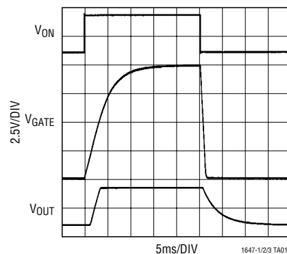
ON/OFF Sequence
