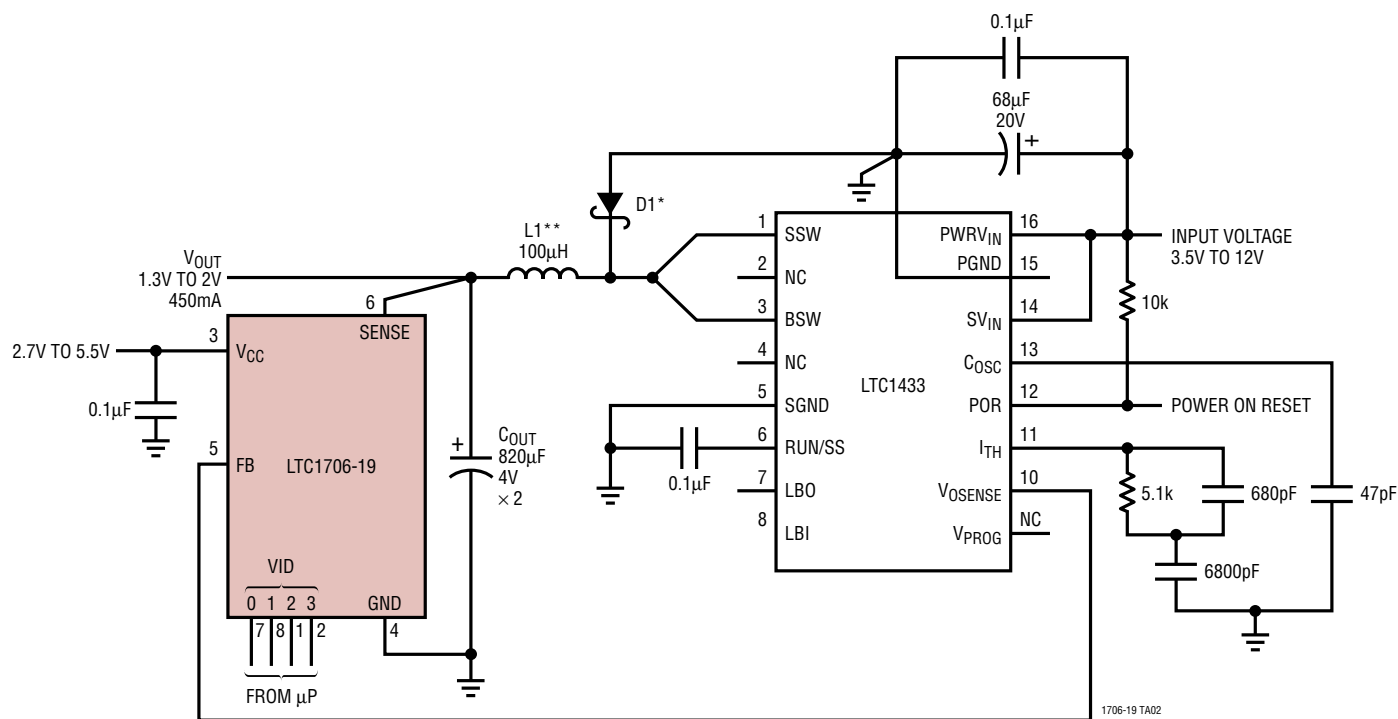
450mA, Low Noise Monolithic Current Mode Step-Down DC/DC Converter
