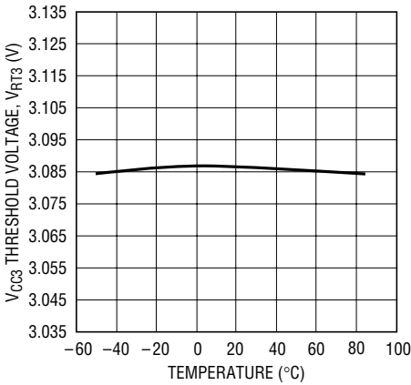
V CC3 Threshold Voltage vs Temperature (All But LTC1728-1.8)
