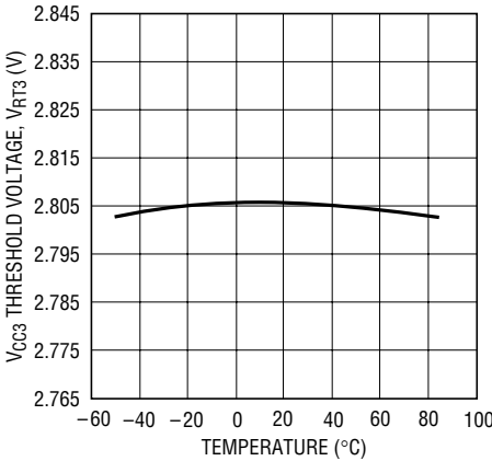
V CC3 Threshold Voltage vs Temperature (LTC1728-1.8)
