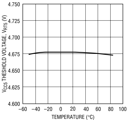
V CC5 Threshold Voltage vs Temperature (LTC1727-5/LTC1728-5)
