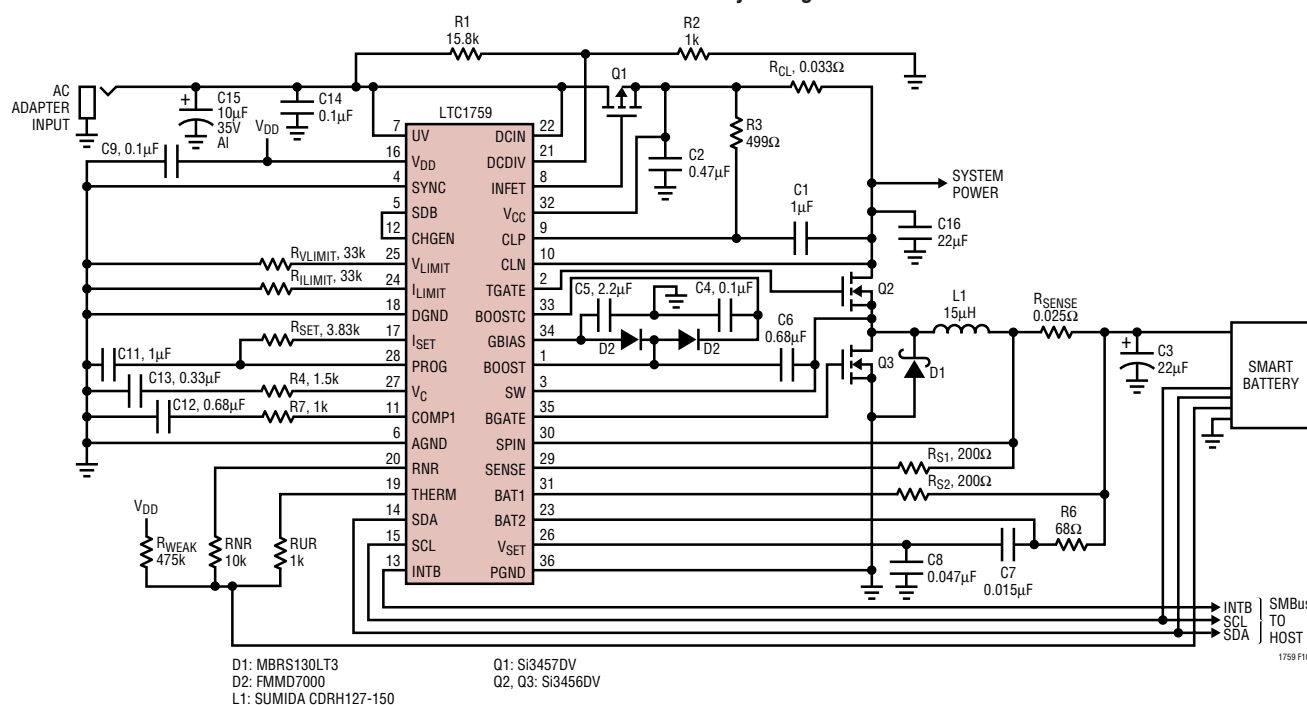
4A SMBus Smart Battery Charger
