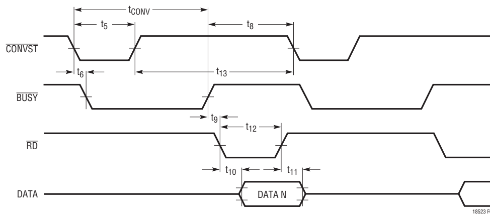
Figure 7. Mode 2 \overline{\text{CONVST}} Starts a Conversion. Data is Read by \text{RD} , \overline{\text{CS}} = 0
