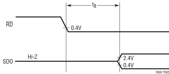
t 8 (SDO Valid After \overline{\text{RD}}\downarrow )
