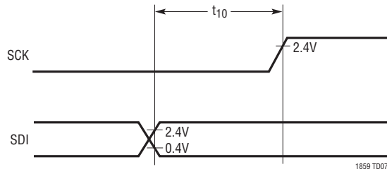
t 10 (SDI Setup Time Before SCK↑)
