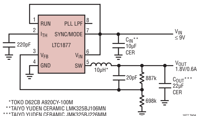
4-to 6-Cell NiCd/NiMH to 1.8V/0.6A Regulator Using All Ceramic Capacitors
