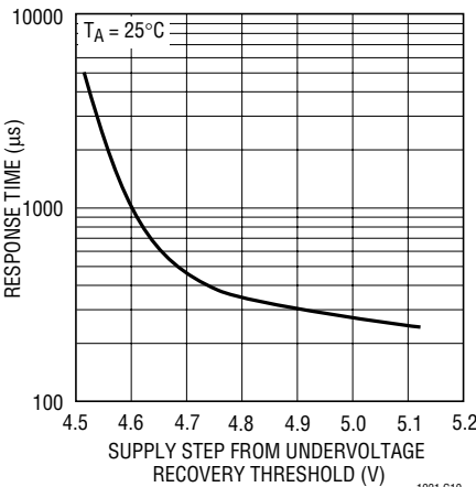
Undervoltage Response Time
