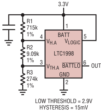
Micropower 2.9V V_{CC} Threshold Detector with 15mV Hysteresis
