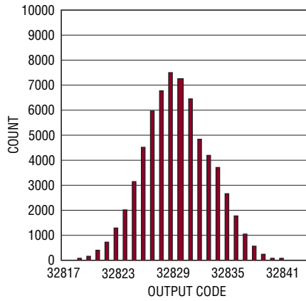
LTC2183: Shorted Input Histogram
