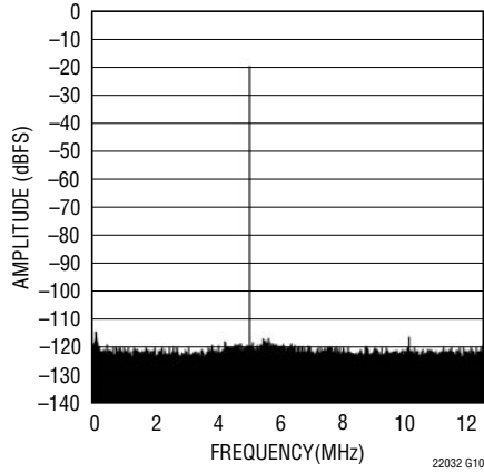
LTC2203: 128K Point FFT, f_{IN} = 5.1\text{MHz} , -20\text{dBFS} , PGA = 0, Internal Dither "On"
