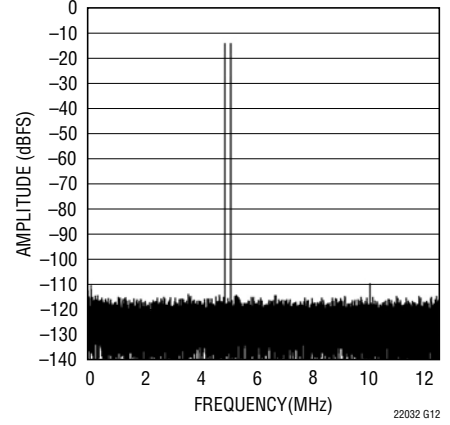
LTC2203: 32K Point 2-Tone FFT, f_{IN} = 4.9\text{MHz} and 30.1\text{MHz} , -15\text{dBFS} , PGA = 0
