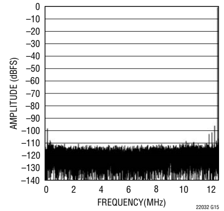
LTC2203: 32K Point FFT, f_{IN} = 12.4\text{MHz} , -1\text{dBFS} , PGA = 0
