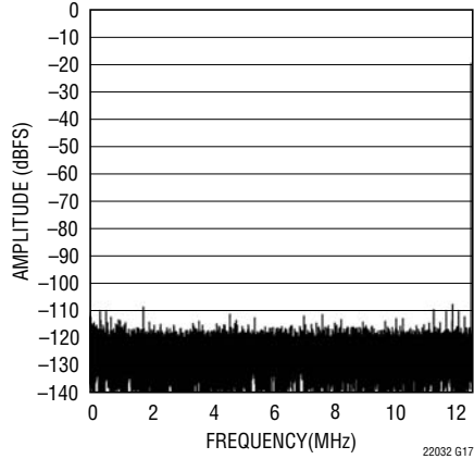
LTC2203: 32K Point FFT, f_{IN} = 12.4\text{MHz} , -20\text{dBFS} , PGA = 0
