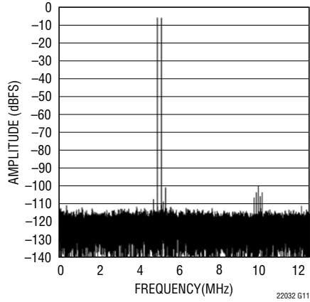
LTC2203: 32K Point 2-Tone FFT, f_{IN} = 4.9\text{MHz} and 30.1\text{MHz} , -7\text{dBFS} , PGA = 0
