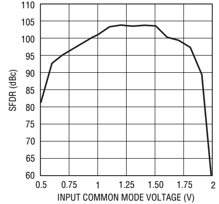
LTC2203: SFDR vs Input Common Mode Voltage, f_{IN} = 5\text{MHz} , -1\text{dBFS} , \text{PGA} = 0
