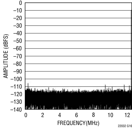
LTC2203: 32K Point FFT, f_{IN} = 12.4\text{MHz} , -10\text{dBFS} , PGA = 0
