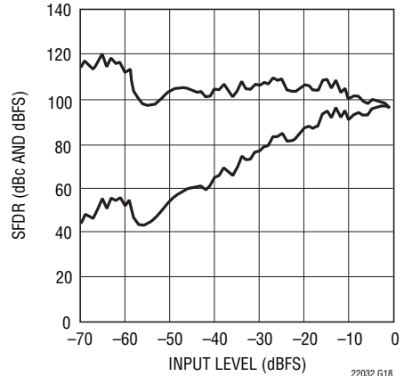
LTC2203: SFDR vs Input Level, f_{IN} = 12.7\text{MHz} , PGA = 0, Dither "Off"
