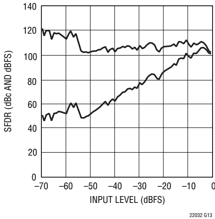
LTC2203: SFDR vs Input Level, f_{IN} = 5\text{MHz} , PGA = 0, Dither "Off"
