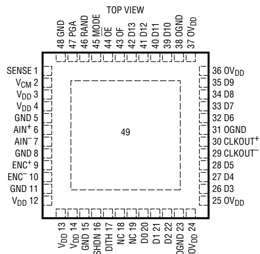
UK PACKAGE 48-LEAD (7mm × 7mm) PLASTIC QFN
