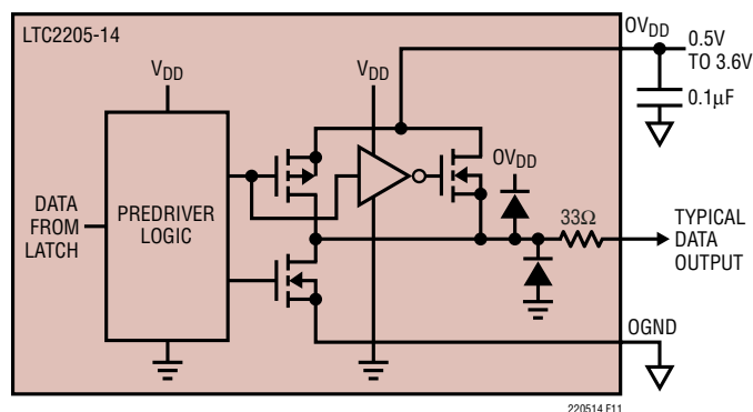
Figure 11. Equivalent Circuit for a Digital Output Buffer
