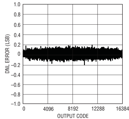
LTC2256-14: Differential Non-Linearity (DNL)
