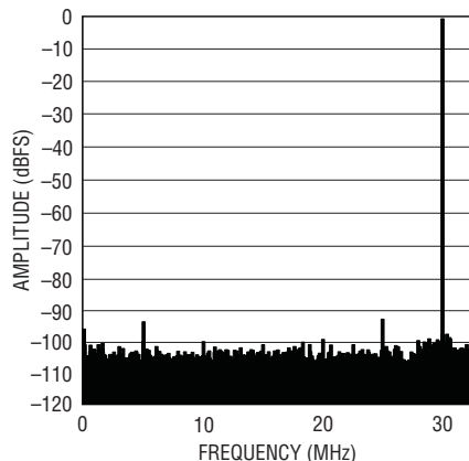
LTC2258-14: 8k Point FFT, f_{IN} = 30\text{MHz} -1dBFS, 65Mps
