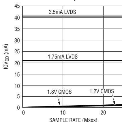
LTC2256-14: I_{OVDD} vs Sample Rate, 5MHz Sine Wave Input, -1dB, 5pF on Each Data Output
