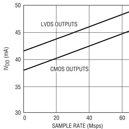
LTC2258-14: I_{VDD} vs Sample Rate, 5MHz Sine Wave Input, -1dB
