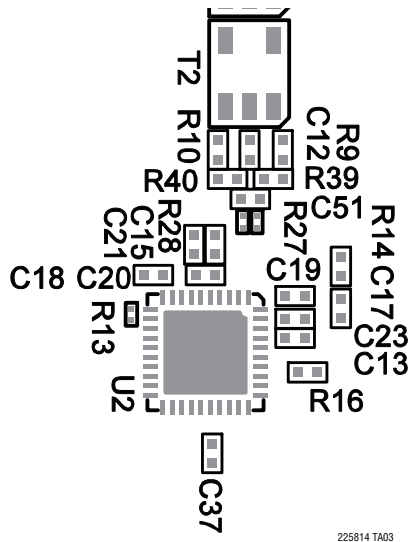
Silkscreen Top
