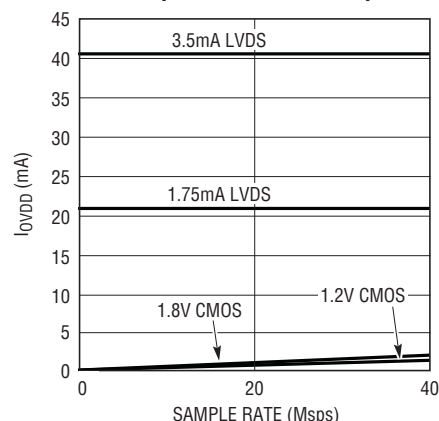
LTC2257-14: I_{O_{VDD}} vs Sample Rate, 5MHz Sine Wave Input, -1dB, 5pF on Each Data Output
