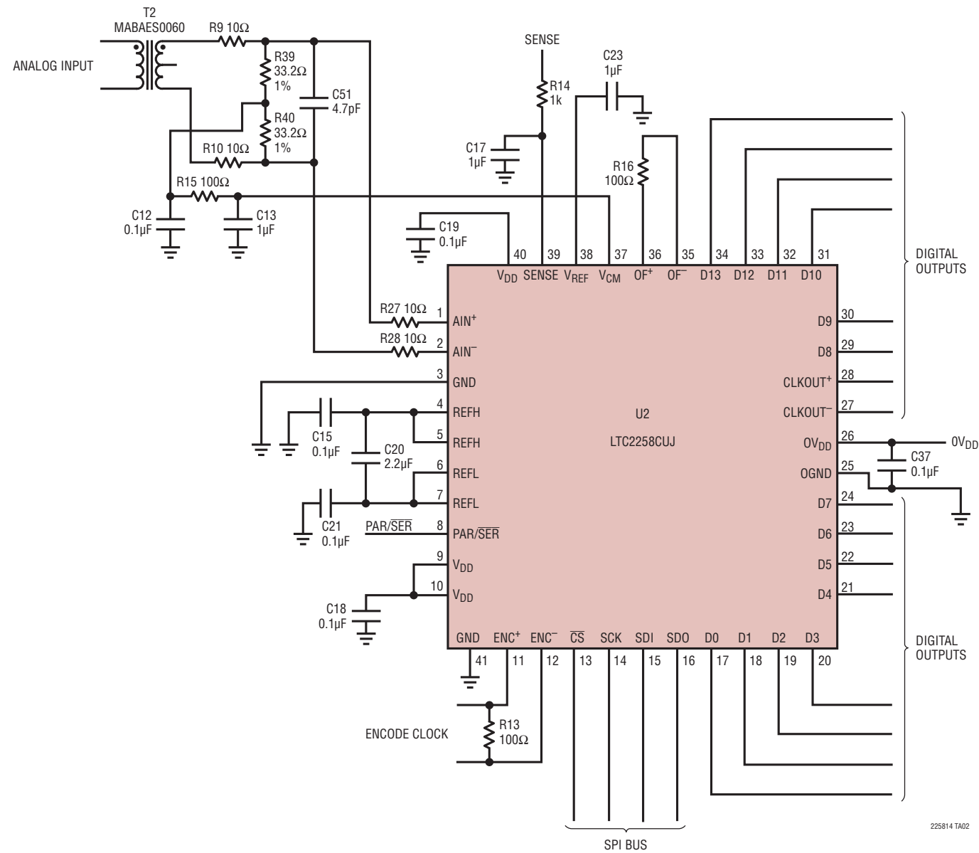
LTC2258 Schematic
