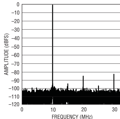
LTC2258-14: 8k Point FFT, f_{IN} = 140\text{MHz} -1dBFS, 65Mps
