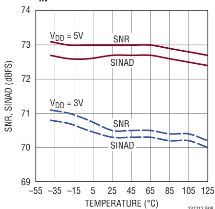
SNR, SINAD vs Temperature, f_{IN} = 259\text{kHz}
