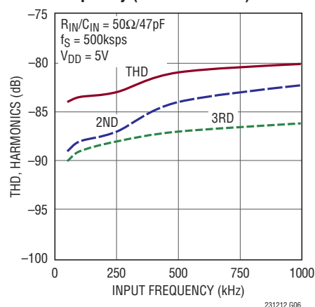
THD, Harmonics vs Input Frequency (50kHz to 1MHz)
