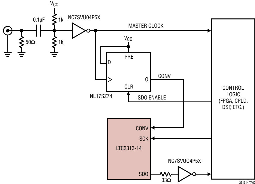
Low Jitter Clock Timing with RF Sine Generator Using Clock Squaring/Level-Shifting Circuit and Re-Timing Flip-Flop
