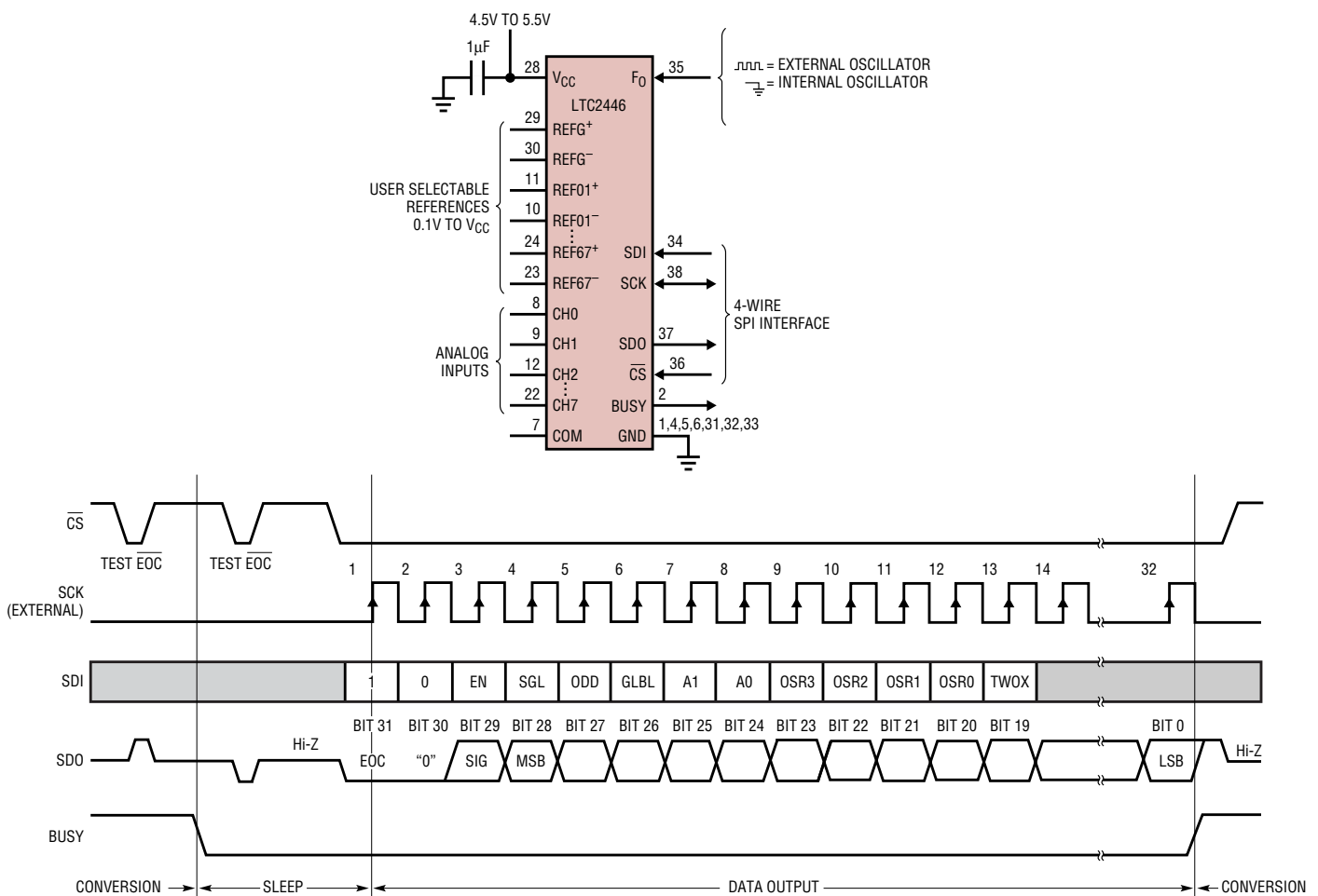
Figure 4. External Serial Clock, Single Cycle Operation
