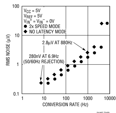
LTC2446 Speed vs RMS Noise
