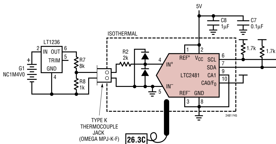
Figure 44. Calibration Setup
