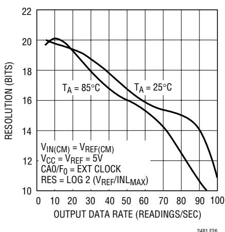
Figure 25. Resolution ( \text{INL}_{\text{MAX}} \leq 1\text{LSB} ) vs Output Data Rate and Temperature
