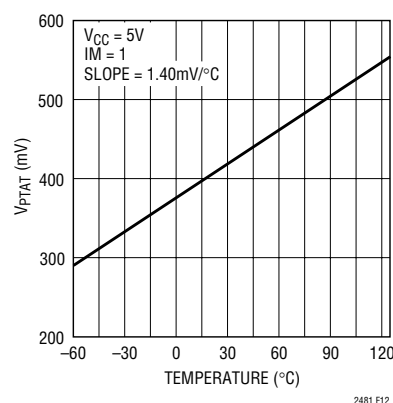
Figure 11. Internal PTAT Signal vs Temperature
