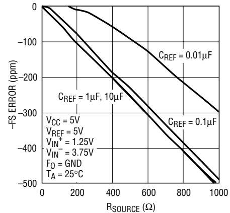
Figure 18. -FS Error vs R_{SOURCE} at V_{REF} (Large C_{REF} )
