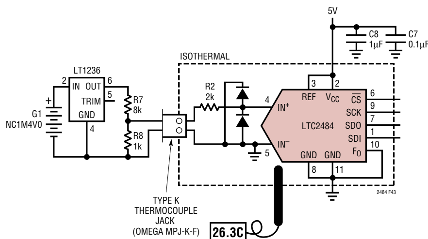
Figure 43. Calibration Setup
