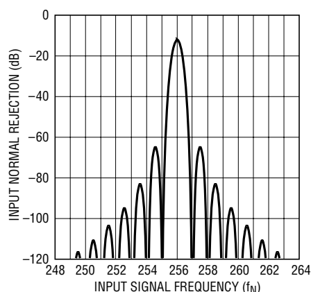
Figure 41. Input Normal Mode Rejection 2x Speed Mode
