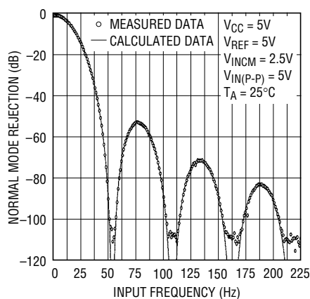
Figure 42. Input Normal Mode Rejection vs Input Frequency, 2x Speed Mode and 50Hz/60Hz Mode
