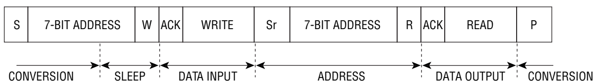
Figure 7. Write, Read, Start Conversion
