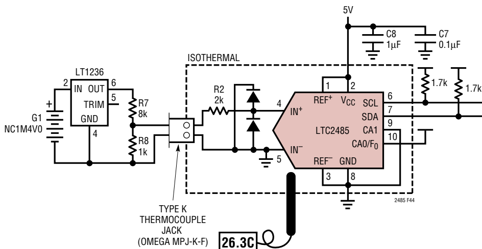
Figure 44. Calibration Setup
