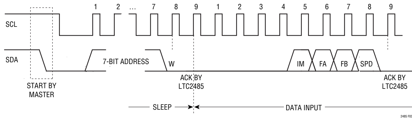
Figure 3. Timing Diagram for Writing to the LTC2485
