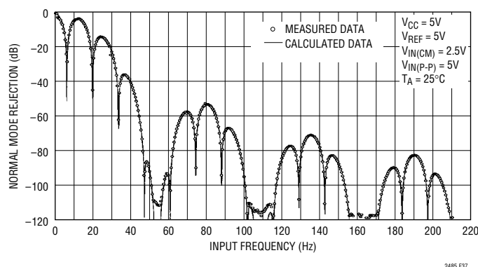
Figure 37. Input Normal Mode Rejection vs Input Frequency with Input Perturbation of 100% Full Scale (50Hz/60Hz Mode)
