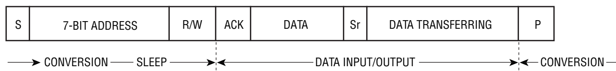
Figure 5. The LTC2485 Conversion Sequence
