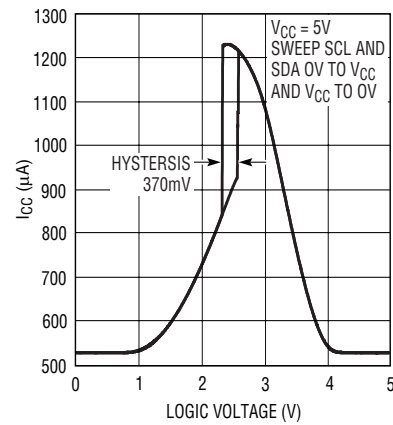
Supply Current vs Logic Voltage
