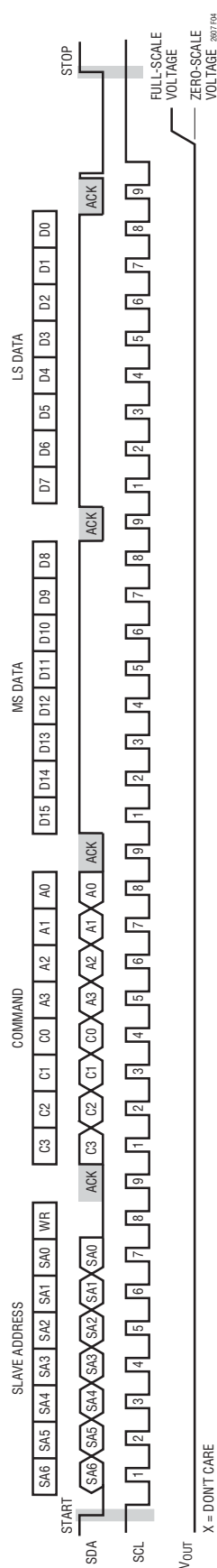
Figure 4. Typical LTC2607 Input Waveform—Programming DAC Output for Full Scale
