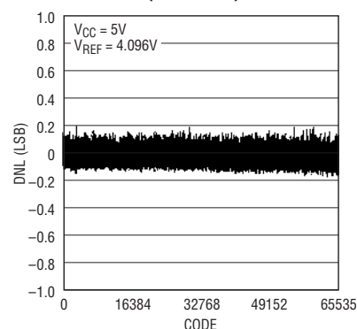
Differential Nonlinearity (LTC2607)
