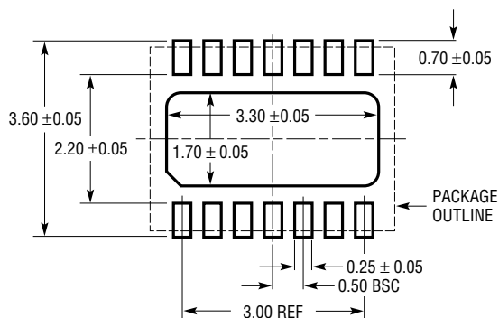
DE Package 14-Lead (4mm × 3mm) Plastic DFN (Reference LTC DWG # 05-08-1708 Rev B)
