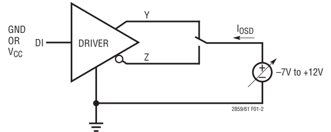
Figure 2. Driver Output Short-Circuit Current
