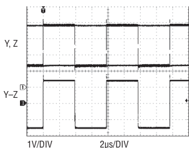
Driver Output at 125kHz into 100 \Omega Resistor
