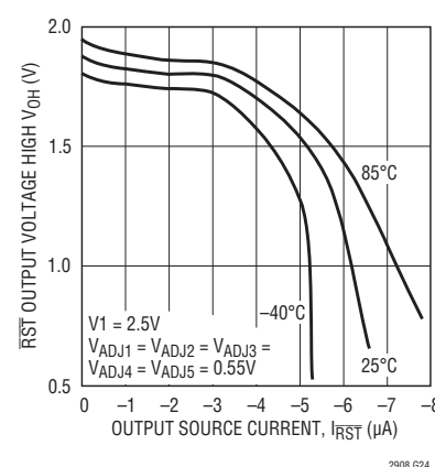
\overline{\text{RST}} Output Voltage High vs \overline{\text{RST}} Output Source Current LTC2908-C1
