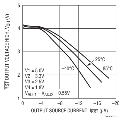
\overline{\text{RST}} Output Voltage High vs \overline{\text{RST}} Output Source Current LTC2908-C1
