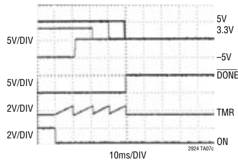
Power-Down Sequence
