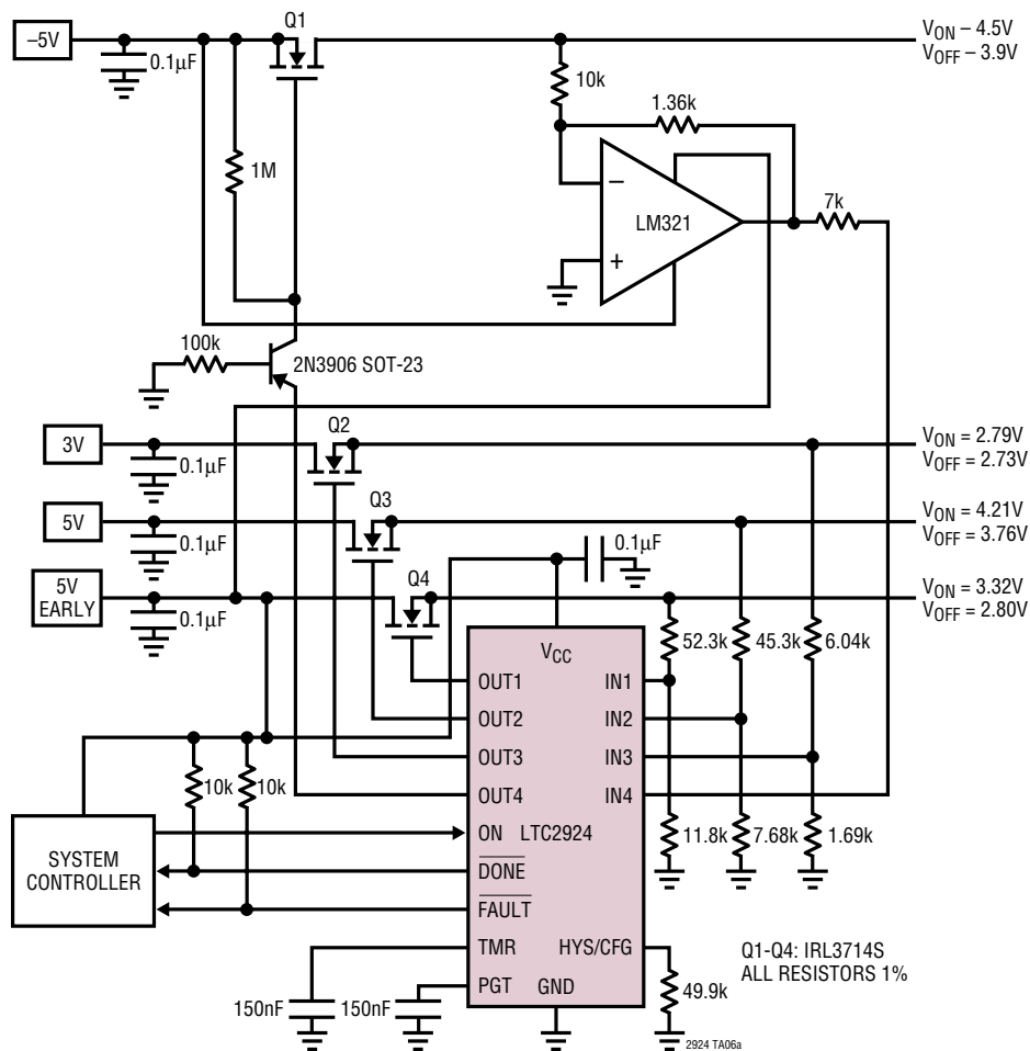
Precision Negative Rail Sequencer
