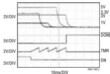
Power-Down Sequence
