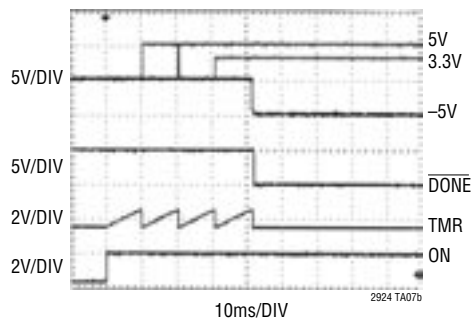
Power-Up Sequence
