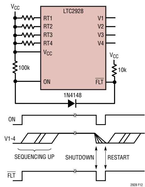
Figure 13. Automatic Restart After Fault
