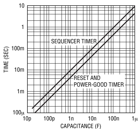
Sequence, Reset and Power-Good Timing vs Capacitance
