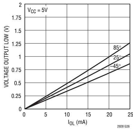
Voltage Output Low vs I_{OL} (CMP, CAS, FLT, DONE, RST, \overline{OV} )
