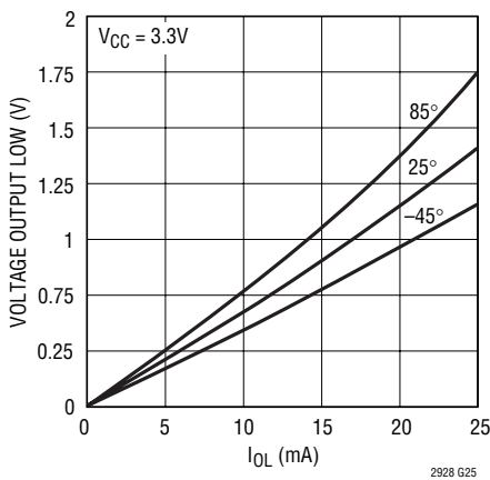
Voltage Output Low vs I_{OL} (CMP, CAS, FLT, DONE, RST, \overline{OV} )
