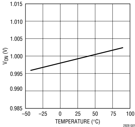
ON Threshold Voltage (Rising) vs Temperature
