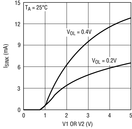
I_{SINK} vs Supply Voltage ( \overline{RST} , COMP_n )
