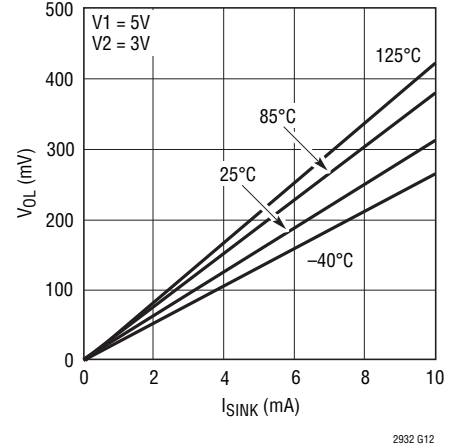
Voltage Output Low vs Output Sink Current ( \overline{RST} , COMP_n )
