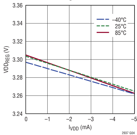
VDD Load Regulation
