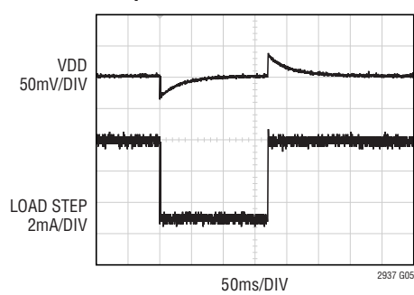
VDD Load Step Transient Response
