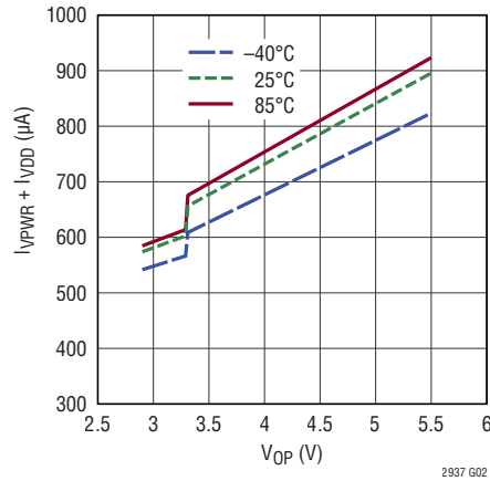
Input Current (VDD tied to VPWR)
