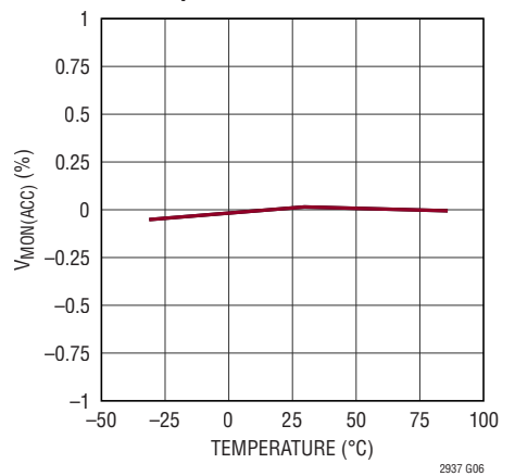
Comparator Threshold Accuracy vs Temperature
