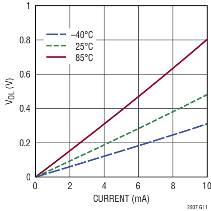
EN/\overline{V_{OL}} vs Output Sink Current
