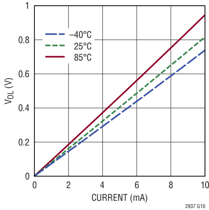
V_{OL} vs Output Sink Current RSTB, FAULT, ALERTB
