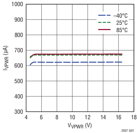
VPWR Input Current (Regulated VDD)
