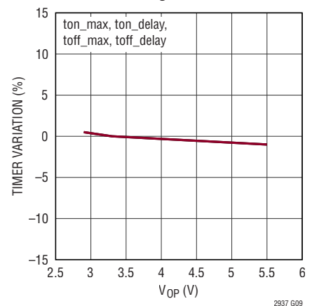
Timer Line Regulation
