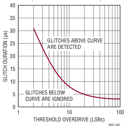
Comparator Glitch Immunity
