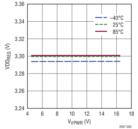
VDD Line Regulation
