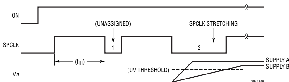
Figure 9. SPCLK Stretching
