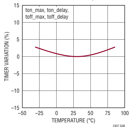
Timer Variation vs Temperature
