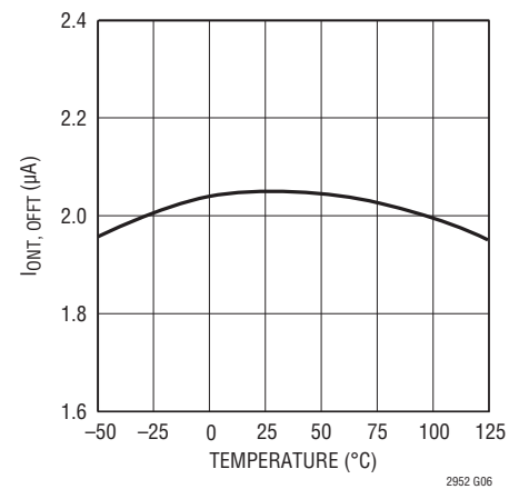
ONT/OFFT Pull-Up/Pull-Down Current vs Temperature
