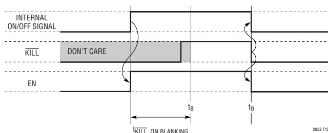
Figure 12. \overline{\text{KILL}} Initiated Shutdown
