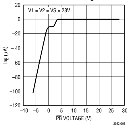
\overline{PB} Current vs \overline{PB} Voltage
