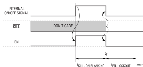
Figure 11. Aborted Power-On Sequence
