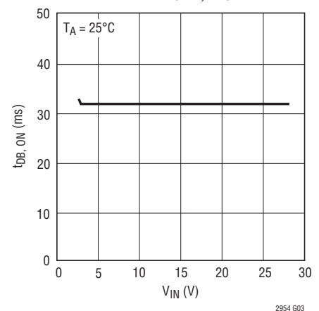
Internal Default Turn-On Debounce Time ( t_{\text{DB,ON}} ) vs V_{\text{IN}}
