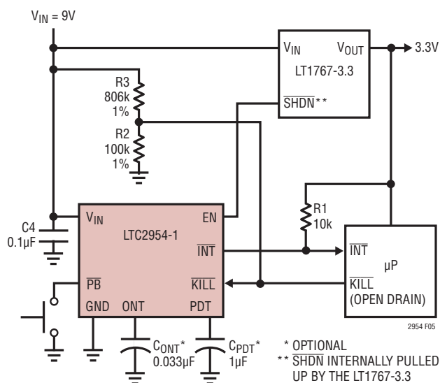
Figure 5. Input Voltage Monitoring with \overline{\text{KILL}} Input
