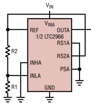
Figure 3a. Rising Edge Built-In Hysteresis by Grounding INH
