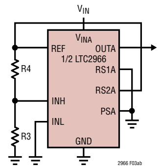
Figure 3b. Falling Edge Built-In Hysteresis by Grounding INL
