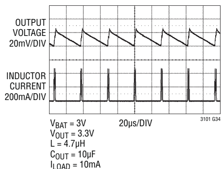
Buck-Boost Burst Mode Ripple
