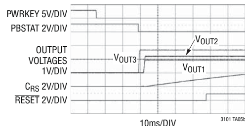
Power-Up Waveforms
