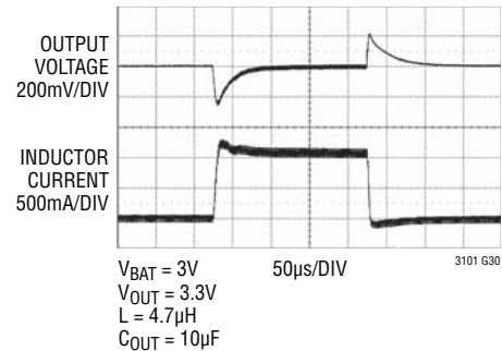
Buck-Boost Load Step, 0mA to 800mA
