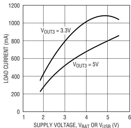
Buck-Boost Maximum Load Current, PWM Mode
