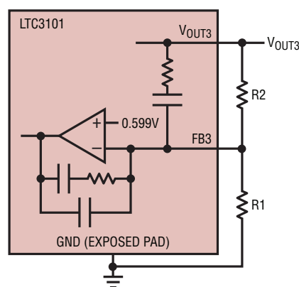
Figure 3. Buck-Boost Error Amplifier and Compensation
