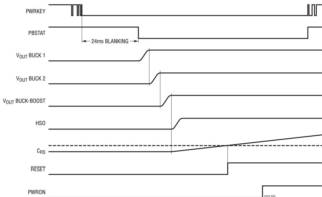
Figure 1. Power-Up Sequence Waveforms
