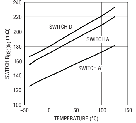
Buck-Boost P-Channel Switch R DS(ON)
