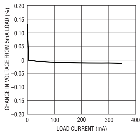
Buck Output Voltage vs Load Current
