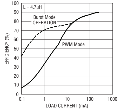
Buck Efficiency USB (5V) to 1.8V
