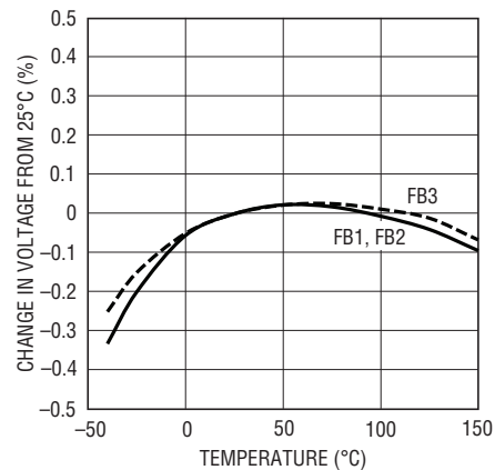
Feedback Voltages
