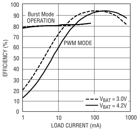
Buck-Boost Efficiency vs Load Current
