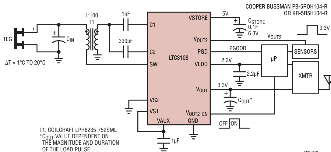
Peltier-Powered Energy Harvester for Remote Sensor Applications
