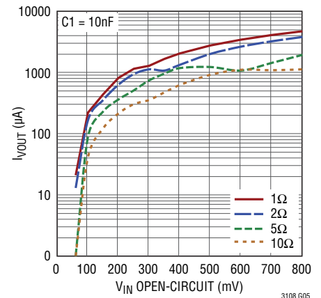
I_{VOUT} vs V_{IN} and Source Resistance, 1:20 Ratio
