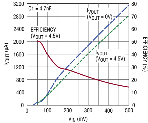
I_{VOUT} and Efficiency vs V_{IN} , 1:50 Ratio Transformer
