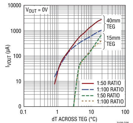
I_{VOUT} vs dT and TEG Size, 1:100 Ratio
