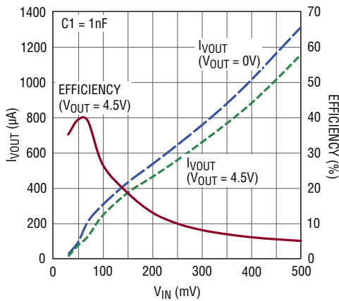
I_{VOUT} and Efficiency vs V_{IN} , 1:100 Ratio Transformer
