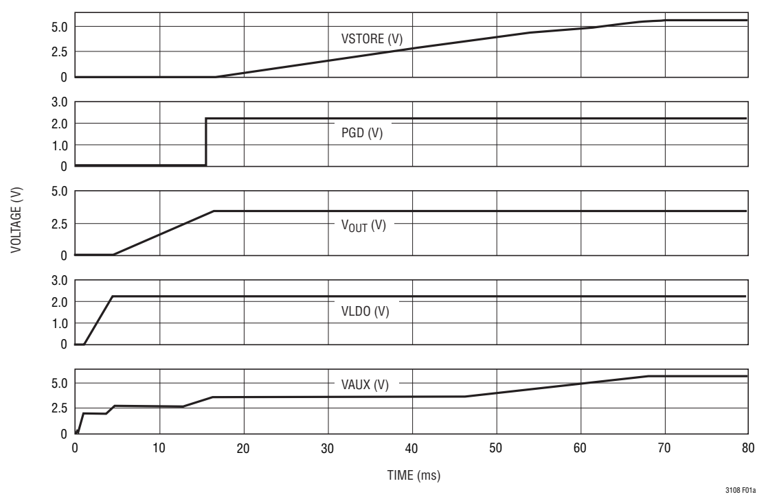
Figure 1. Output Voltage Sequencing with V_{OUT} Programmed for 3.3V (Time Not to Scale)
