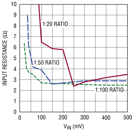
Input Resistance vs V_{IN} ( V_{OUT} Charging)
