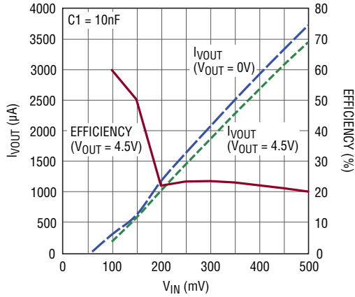
I_{VOUT} and Efficiency vs V_{IN} , 1:20 Ratio Transformer
