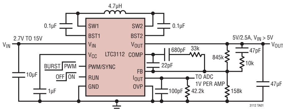
5V, 750kHz Wide Input Voltage Buck-Boost Regulator
