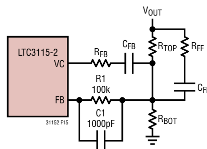
Figure 15. R1 and C1 are Recommended if R_{TOP} < 1M\Omega
