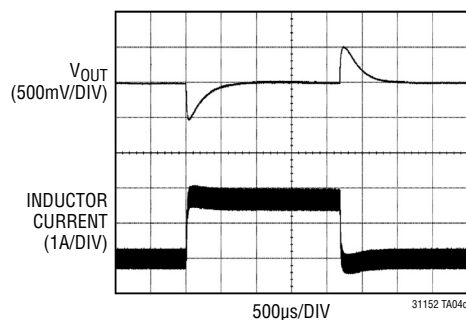
0A to 1.5A Load Step, V_{IN} = 24V
