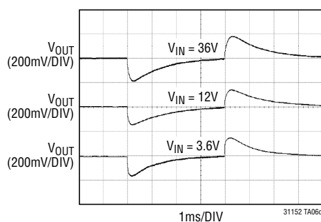
Output Voltage Transient Response, 600mA Load Step, Powered from Automotive Input
