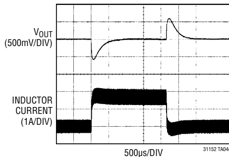
0A to 1.5A Load Step, V_{IN} = 40V
