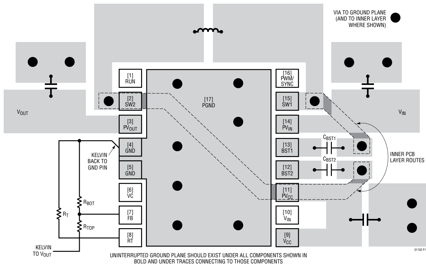
Figure 16. PCB Layout Recommended for the DHD Package
