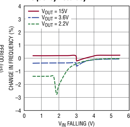
Frequency Accuracy
