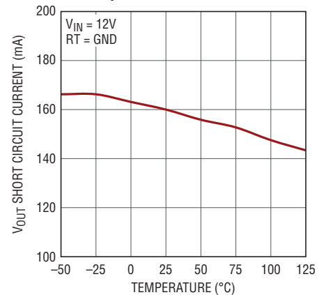
VOUT Short Circuit Current vs Temperature
