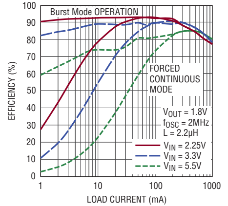
1A Buck Efficiency vs I_{LOAD}
