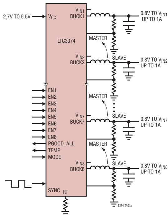
8-Channel 1A Multioutput Buck Regulator
