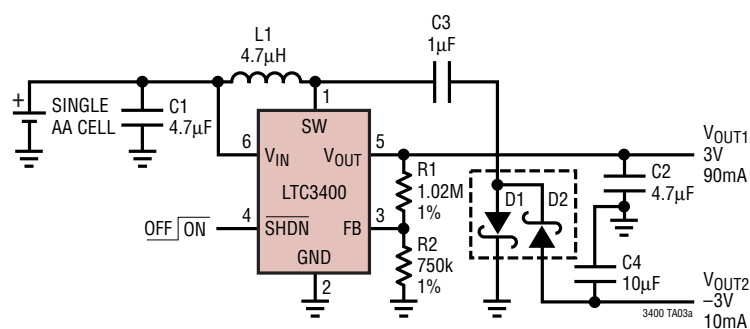
Single Cell AA Cell to \pm 3V Synchronous Boost Converter
