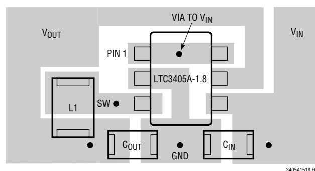
Figure 5. LTC3405A-1.8 Suggested Layout
