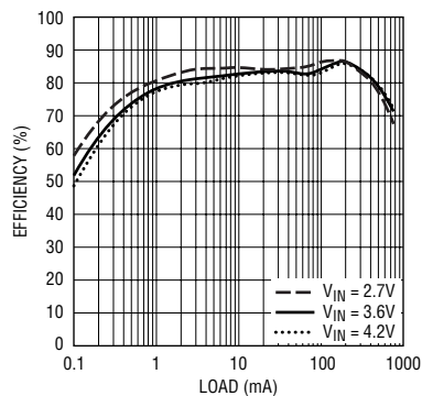
LTC3406-1.2 Efficiency
