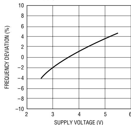
Oscillator Frequency Deviation vs Supply Voltage
