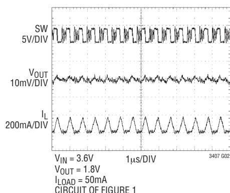
Pulse-Skipping Mode
