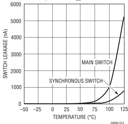
Switch Leakage vs Temperature V_{IN} = 5.5\text{V}
