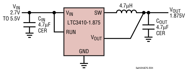
Figure 1. High Efficiency Step-Down Converter
